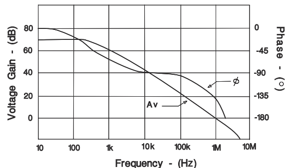
Figure 6-2. Error Amplifier Open-Loop Frequency Response
