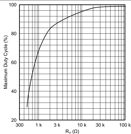
Figure 7-5. Maximum Duty Cycle vs Timing Resistance
