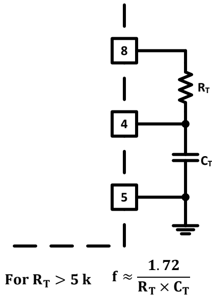
Figure 7-6. Oscillator Section
