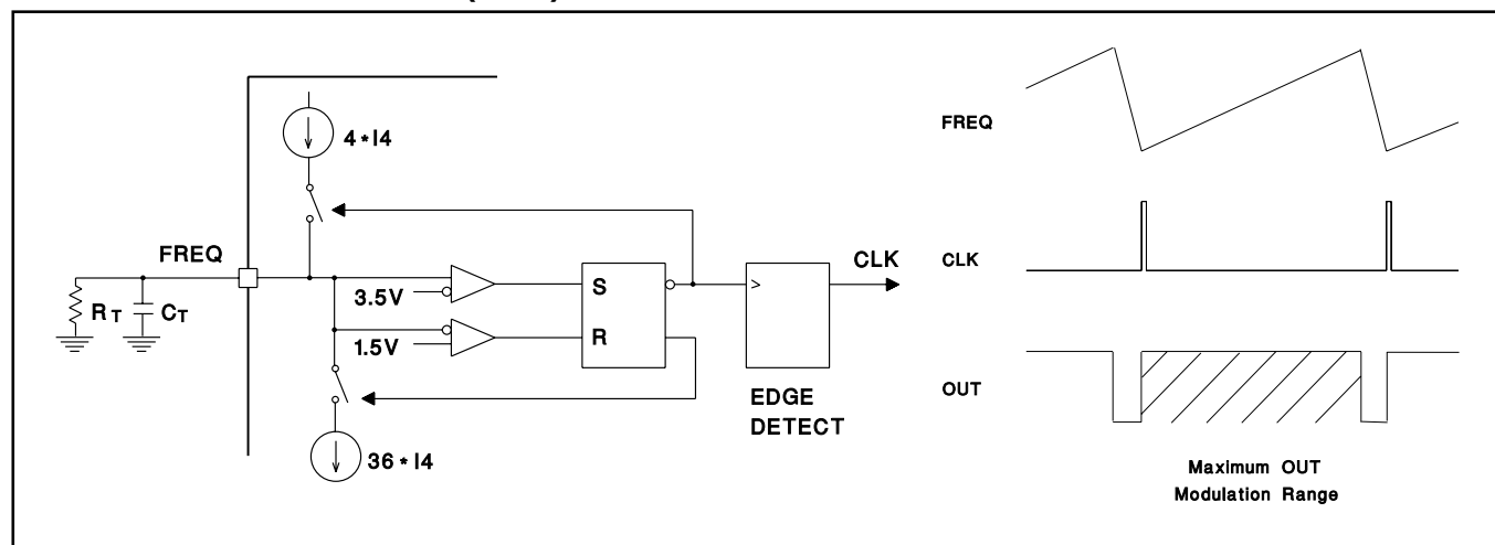
Figure 3. Clock generator.
