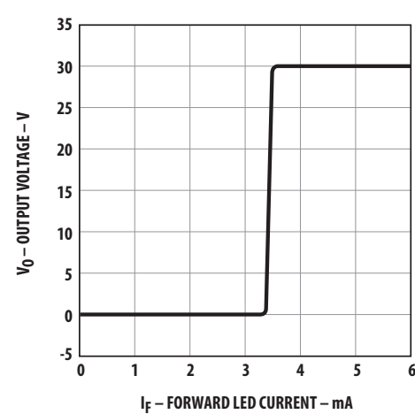
Figure 15 Transfer Characteristics
