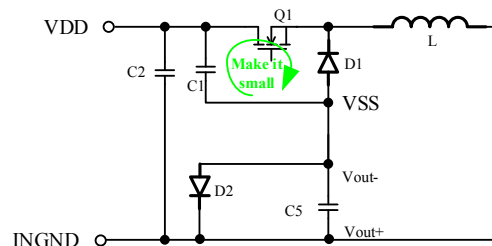
Figure 5—Buck-boost layout without VSS capacitor
