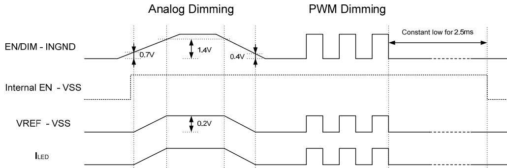
Figure 3— Internal EN Shut-down Delay Function Waveform Diagram
