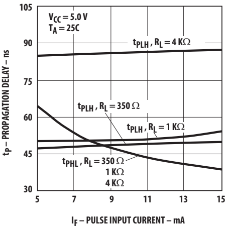
Figure 9 Propagation Delay vs. Pulse Input Current
