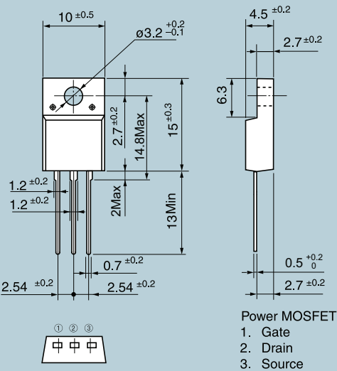
TO-220F (SLS)
