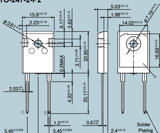
TO-247-2-P2
