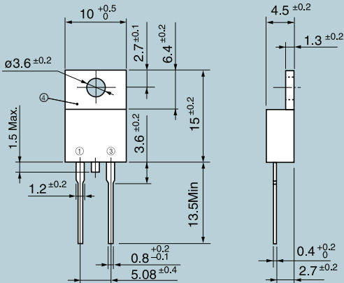
TO-220-2
