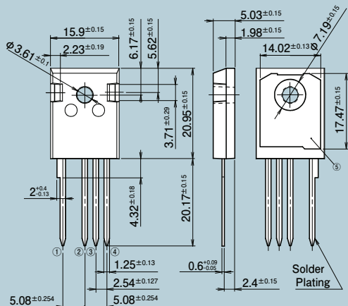
TO-247-4-P2
