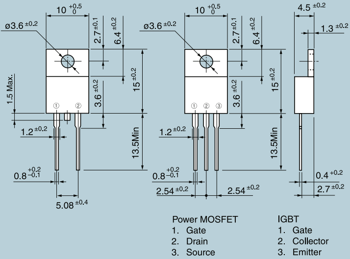
TO-220AB
