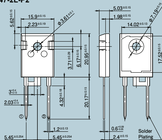
TO-247-2L-P2
