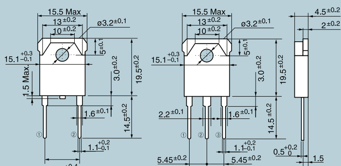
TO-3P
