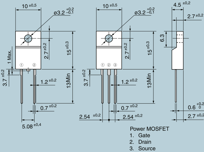
TO-220F-2
