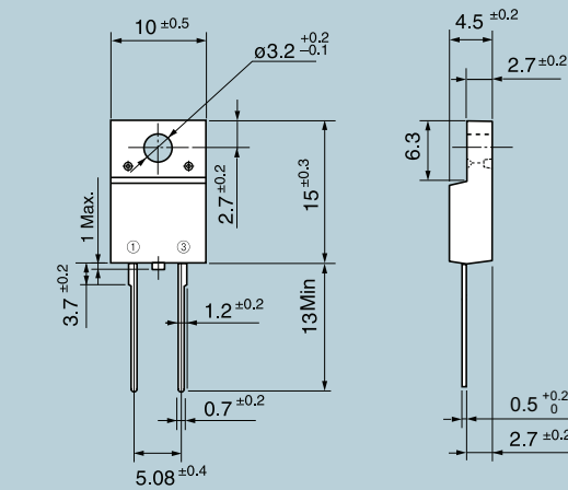
TO-220F-2
