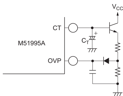
Figure 37 Application Circuit Diagram to Keep the Non-Operating Condition when Over Load Current Condition will Continue for Specified Duration
