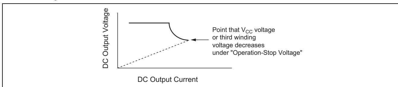
Figure 35 Over Current Limiting Curve on Fly Back System
