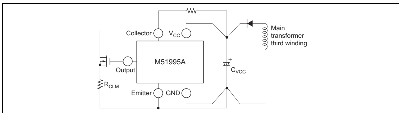
Figure 24 How to Design the Conductor-pattern of Type M51995A on PC Board (schematic example)
