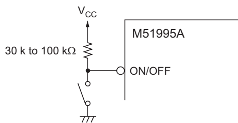
Figure 18 Connecting of ON/OFF Terminal
