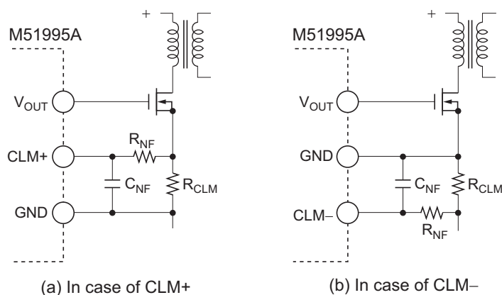
Figure 10 How to Connect Current Limit Circuit
