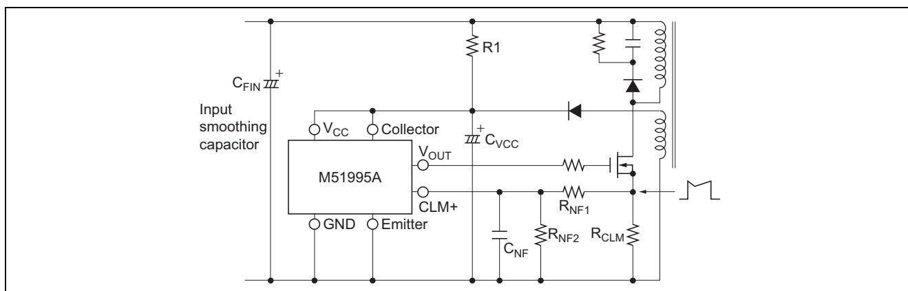
Figure 29 Peripheral Circuit Diagram of CLM+ Terminal
