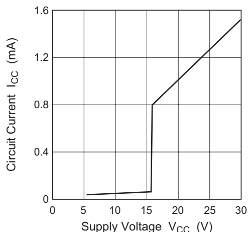
Figure 19 I_{CC} vs. V_{CC} in OFF State
