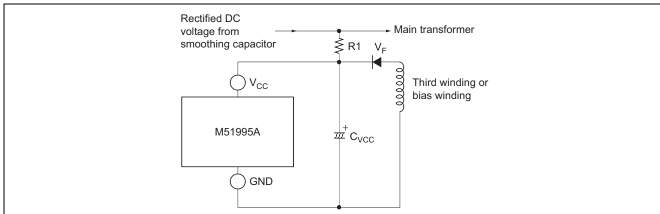
Figure 22 Start-up Circuit Diagram (when it is not necessary to set the start and stop input voltage)
