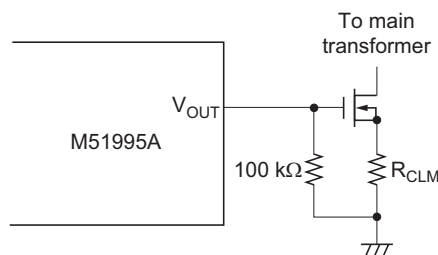
Figure 38 Circuit Diagram to Prevent the MOS FET Gate Potential Rising
