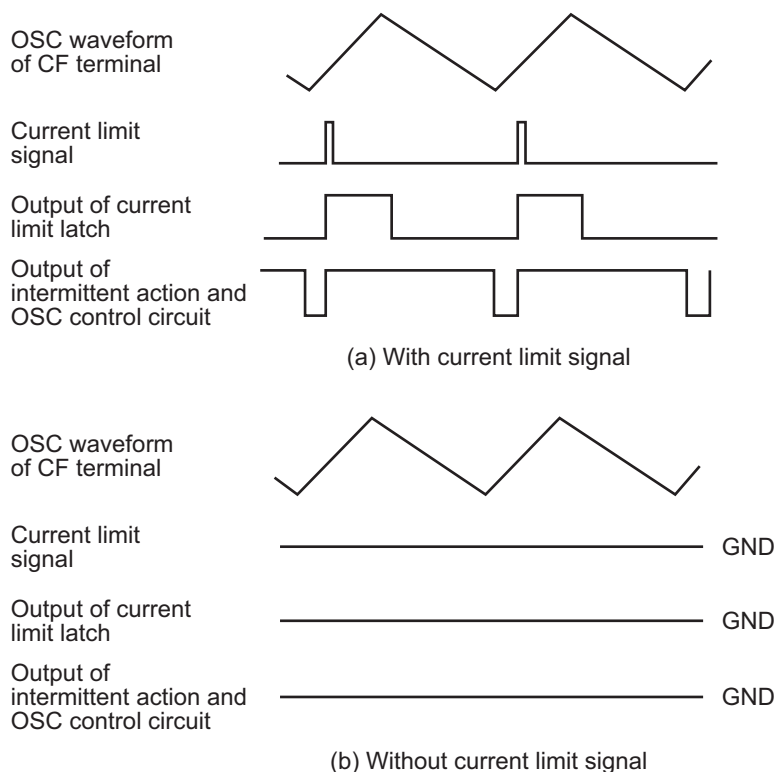
Figure 11 Timing Chart of Intermittent and OSC Control Circuit
