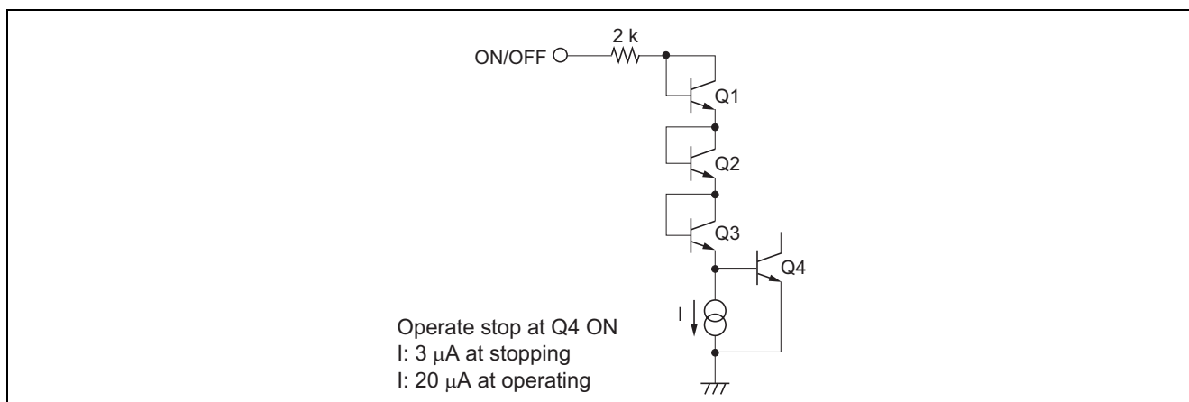
Figure 17 ON/OFF Circuit
