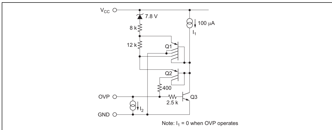
Figure 20 Detail Diagram of OVP Circuit
