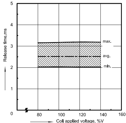
Release time
