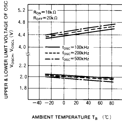
UPPER &amp; LOWER LIMIT VOLTAGE OF OSC VS. AMBIENT TEMPERATURE
