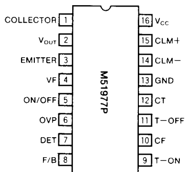
Outline 16P4
