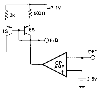
Fig. 18 Equivalent circuit diagram of voltage detector
