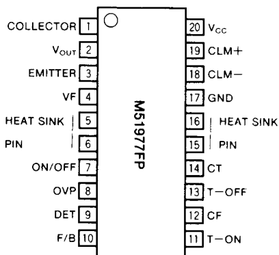
Outline 20P2N
