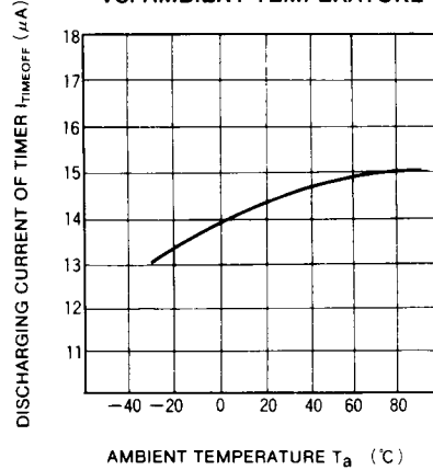
DISCHARGING CURRENT OF TIMER VS. AMBIENT TEMPERATURE
