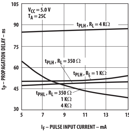
Figure 9 Propagation Delay vs. Pulse Input Current
