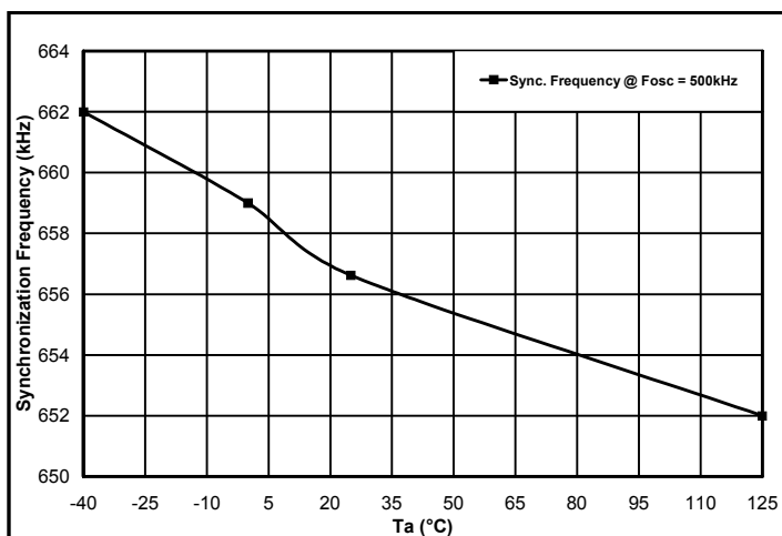
Synchronization Frequency vs. Temperature
