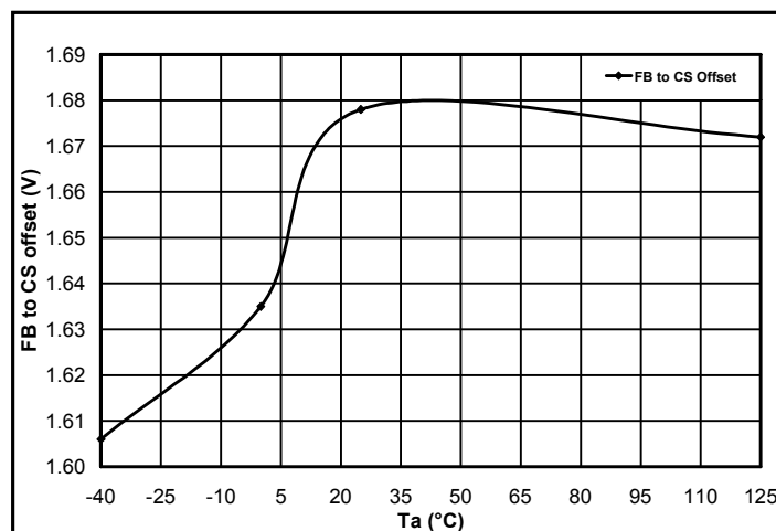
FB to CS Offset vs. Temperature
