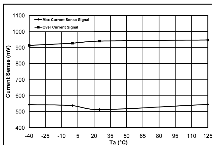
Current sense vs. Temperature
