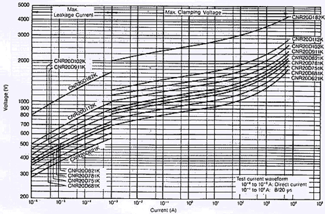
V-I Curve (CNR20D621K to CNR20D182K)
