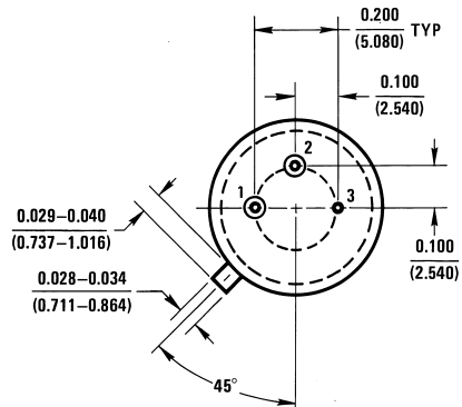
TO-39 Metal Can Package (H) NS Package Number H03A
