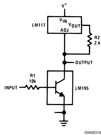
High Gain Amplifier
