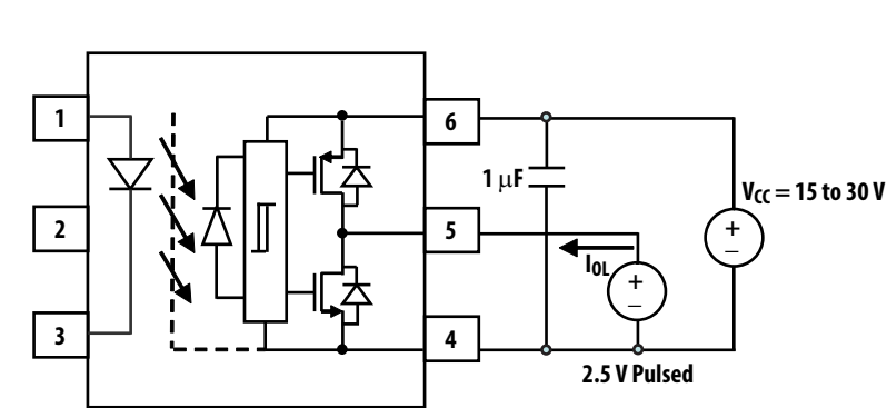
Figure 21 I_{OL} Test Circuit
