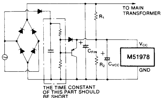
Fig. 24 Peripheral circuit diagram of CLM + terminal
