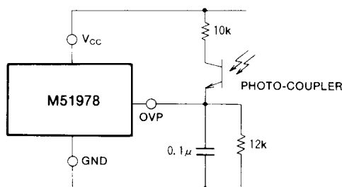
(2) Application circuit to make the OVP-reset time fast
