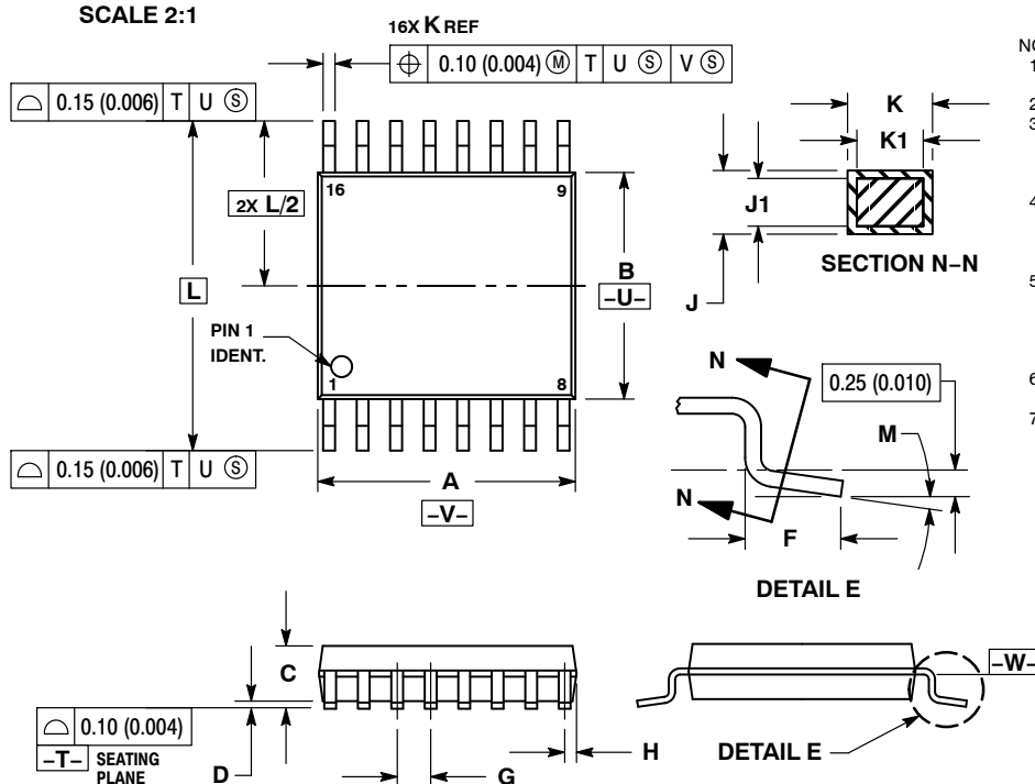
TSSOP-16 WB CASE 948F ISSUE B
